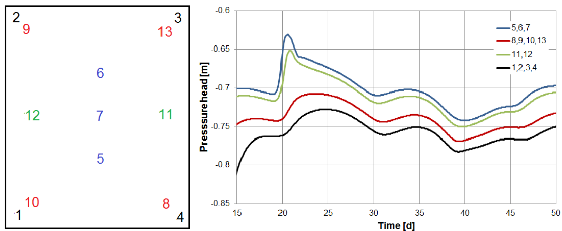
Figure 4. Comparison of possible placement options for measurement devices in 1.5 m depth comparing the effect of centered devices vs. devices at the side, the
