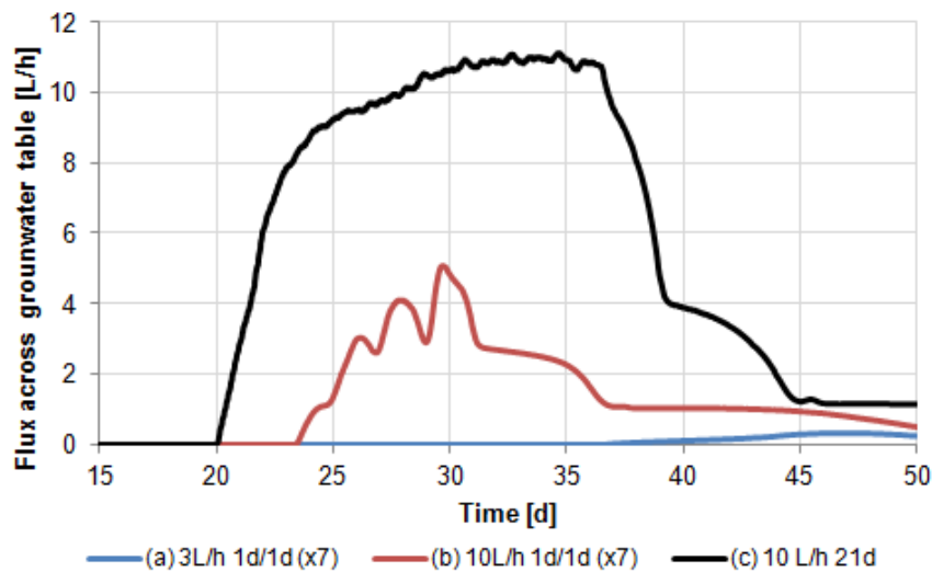
Figure 7. Total value of the boundary flux across the lower boundary (groundwater table) for three different scenarios
