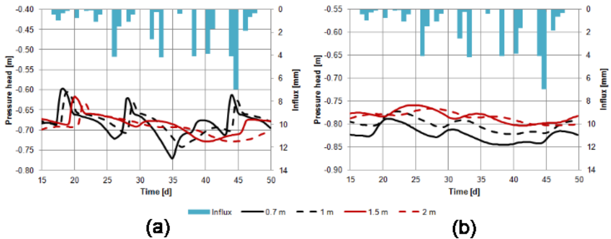
Figure 3. Pressure head distribution (a) in the center and (b) at the side underneath the infiltration unit showcasing water movement in different depths below surface.
