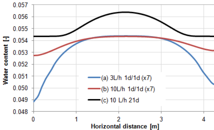
Figure 6. Cross section of horizontal moisture distribution of three different infiltration scenarios simulated 5 m below surface after 50 days. Location of cross section is marked in Figure 5c with a black line.
