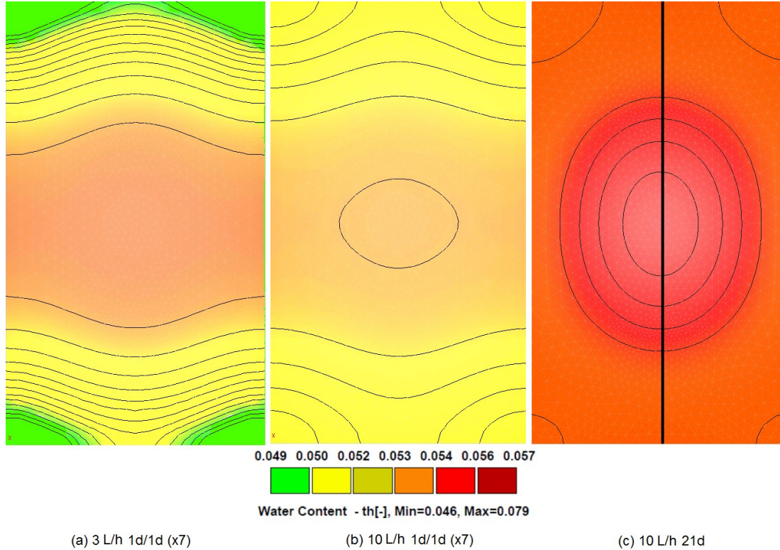
Figure 5. Horizontal water content distribution of three different infiltration scenarios simulated 5 m below surface after 50 days.
