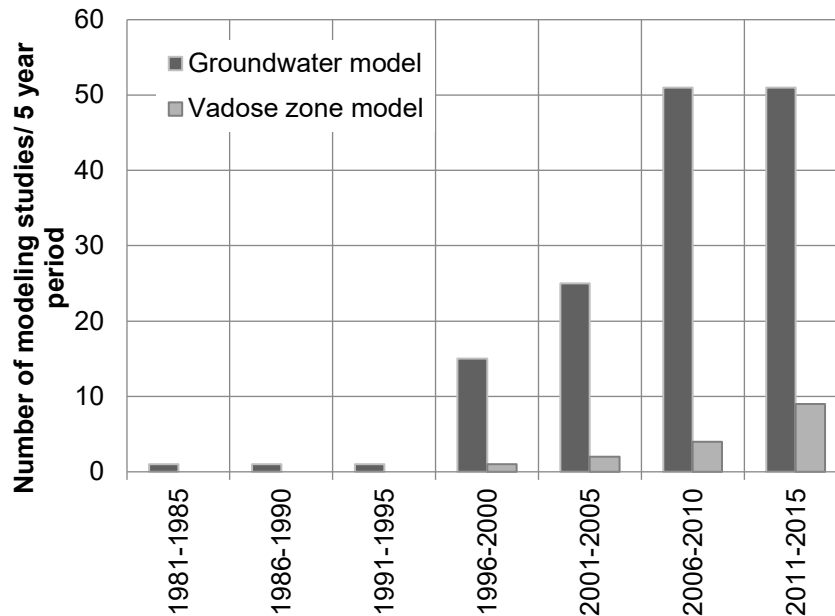
Figure 1. Comparison of the historical application of vadose zone vs. groundwater flow models for MAR evaluation (after Ringleb et al. 2016)
